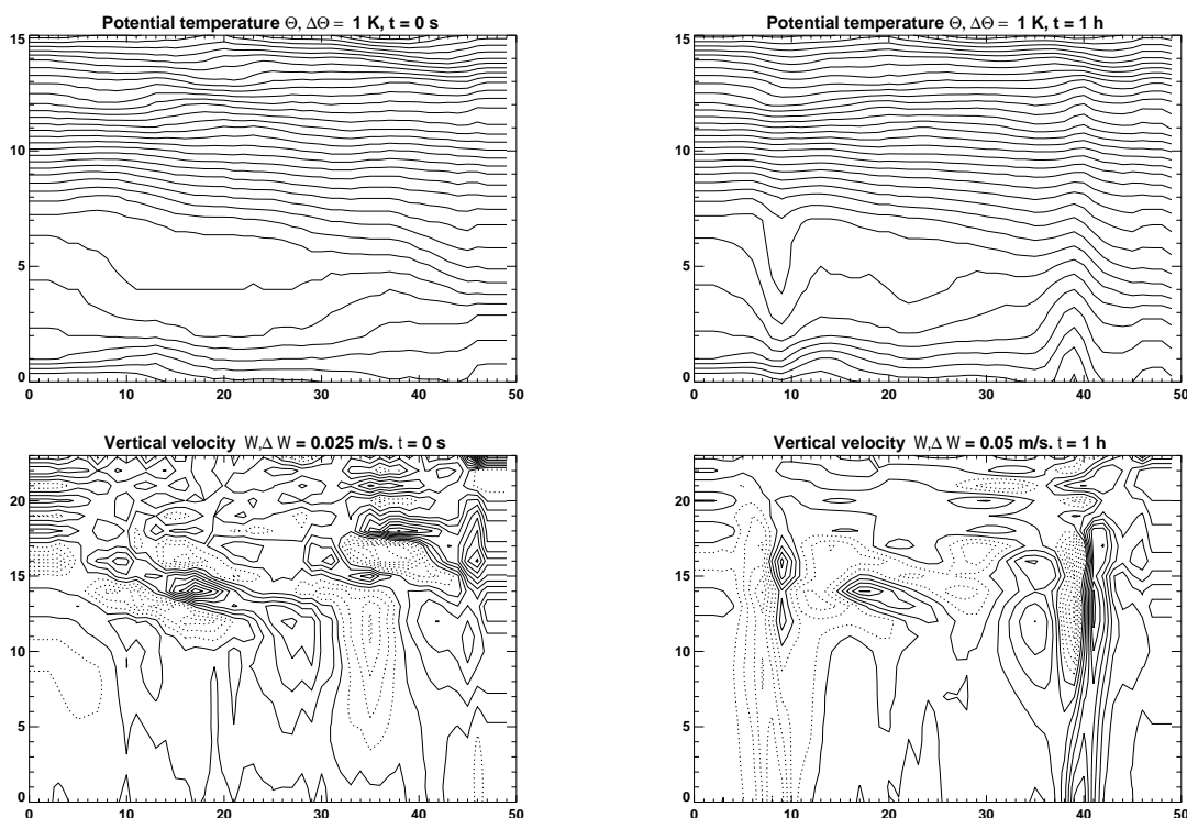
Fig. Potential temperature \theta (upper panels) and vertical velocity w (lower panels) in vertical plane j = 25 in the initial moment (left panels) and after 1 h (120 steps of integration).
