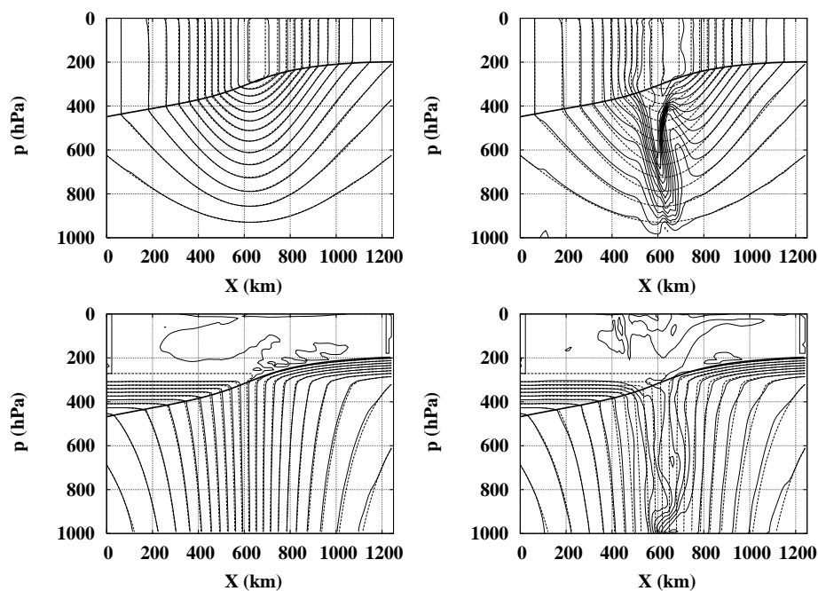
Fig. 10. Zonal ( y = 0 ) vertical cross sections of the meridional wind component (top panels) and temperature fluctuation (bottom panels) for stable integration mode (left panels, \Delta t = 300 s, 24 h development) and for unstable integration mode (right panels, \Delta t = 420 s, 6 h development). Tropopause location is marked by the heavy line. Dotted contours mark the exact solution. Isotachs and isotherms are drawn with 5 \text{ m s}^{-1} and 2.0 \text{ K} interval, respectively.
